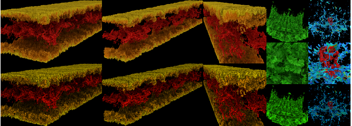
Figure 1: All images rendered with our speculative ray tracing technique. First three columns: a massive channel-flow turbulence DNS dataset. Last two columns: an RM fluid instability dataset and an Enzo Astrophysics AMR dataset (left and right). The number of triangles from left to right: DNS2 (1.8 billion), DNS1-side and DNS1-back (0.9 billion), RM (108 million), and Enzo (8 million). Five images on the bottom row show ambient occlusion shading, and the rest show three-bounce path tracing. For all datasets, 32 samples per pixel were used to render images at 1024 \times 1024 resolution, and one diffuse ray and 16 shadow rays were generated at every hit point. Using Stampede2 Skylake at the Texas Advanced Computing Center, each node with 192 GB memory, at least eight nodes are required to render the DNS dataset with speculation enabled.
